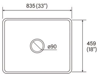
A-3318N Farmhouse Sink Size: 835x459x254 mm
